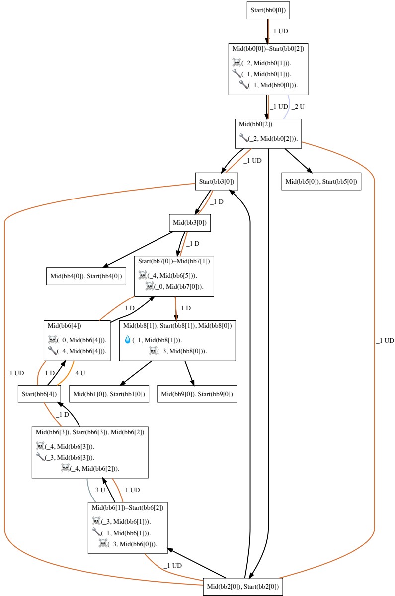
Figure 6.2.1: A graph representation of the the variable liveness calculation results, with relevant Polonius facts as they occur (a droplet symbolising \text{var\_drop\_used}(V, \_) , a wrench \text{var\_used}(V, \_) , and a skull and crossbones symbolising \text{var\_defined}(V, \_) ). Variables are named by prefixing underscores, and edges annotated with the propagated live variable and its liveness type(s) ( D rop or U se). The source code is one of the test cases for drop-liveness.
